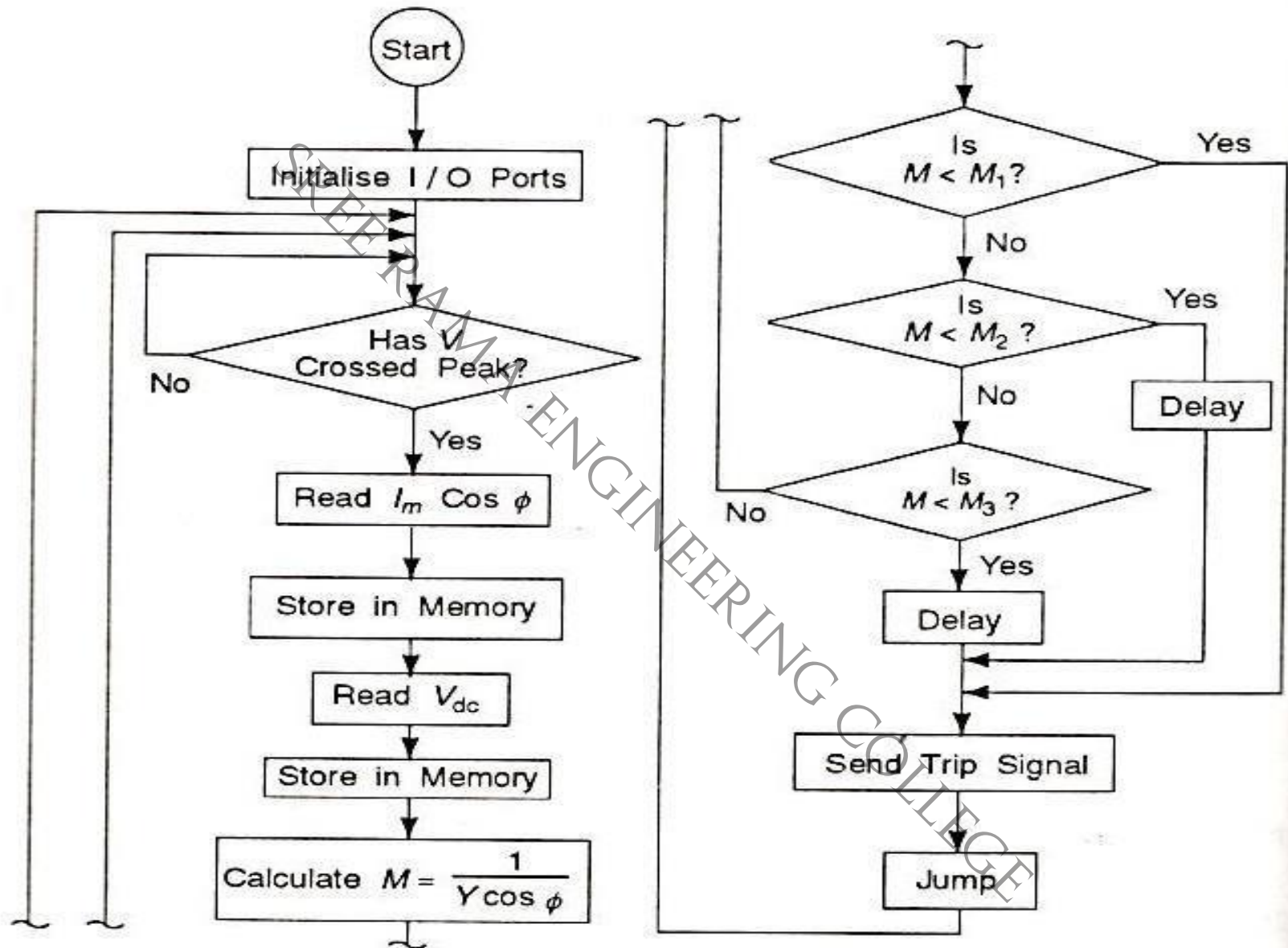
FIGURE 8.19 Program flowchart for mho relay
