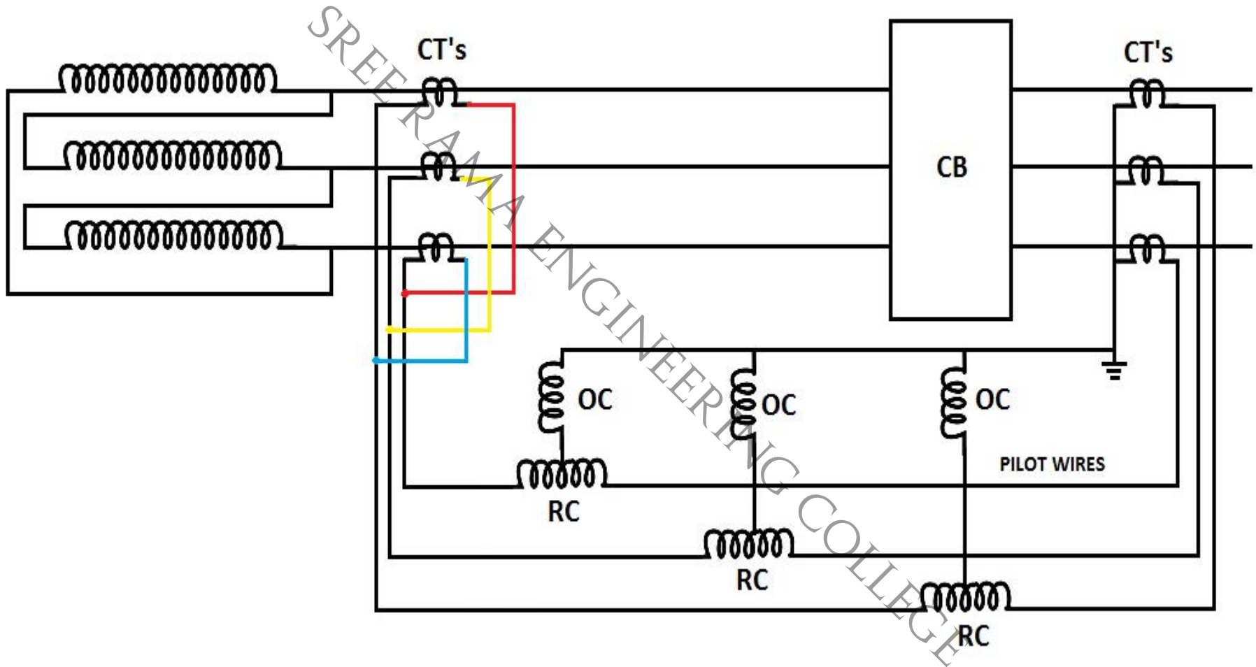
Fig. 2. % Differential protection of a DELTA connected Alternator
