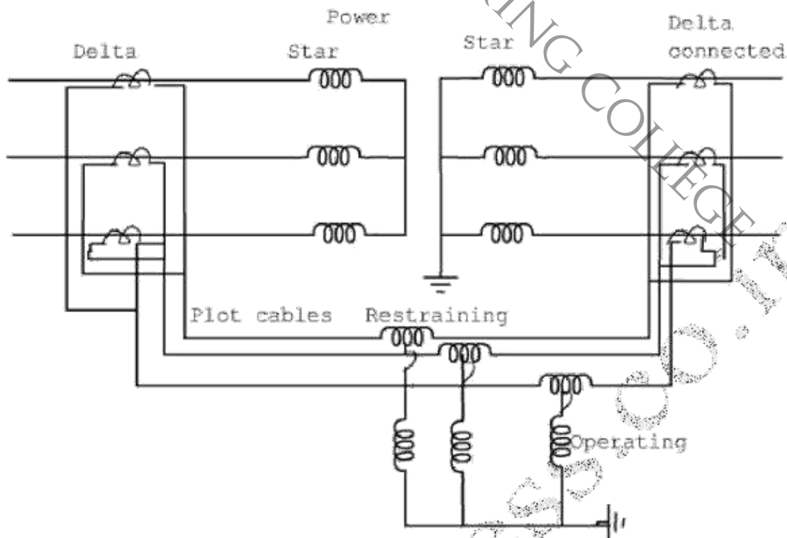
Fig: Differential protection of star-star
