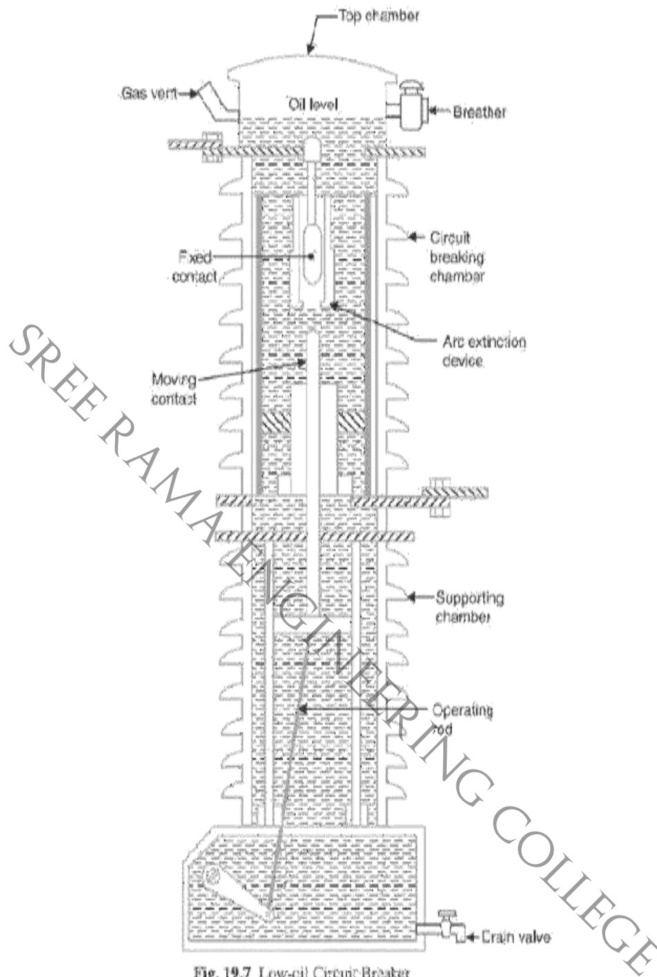
Fig. 19.7 Low-oil Circuit Breaker
