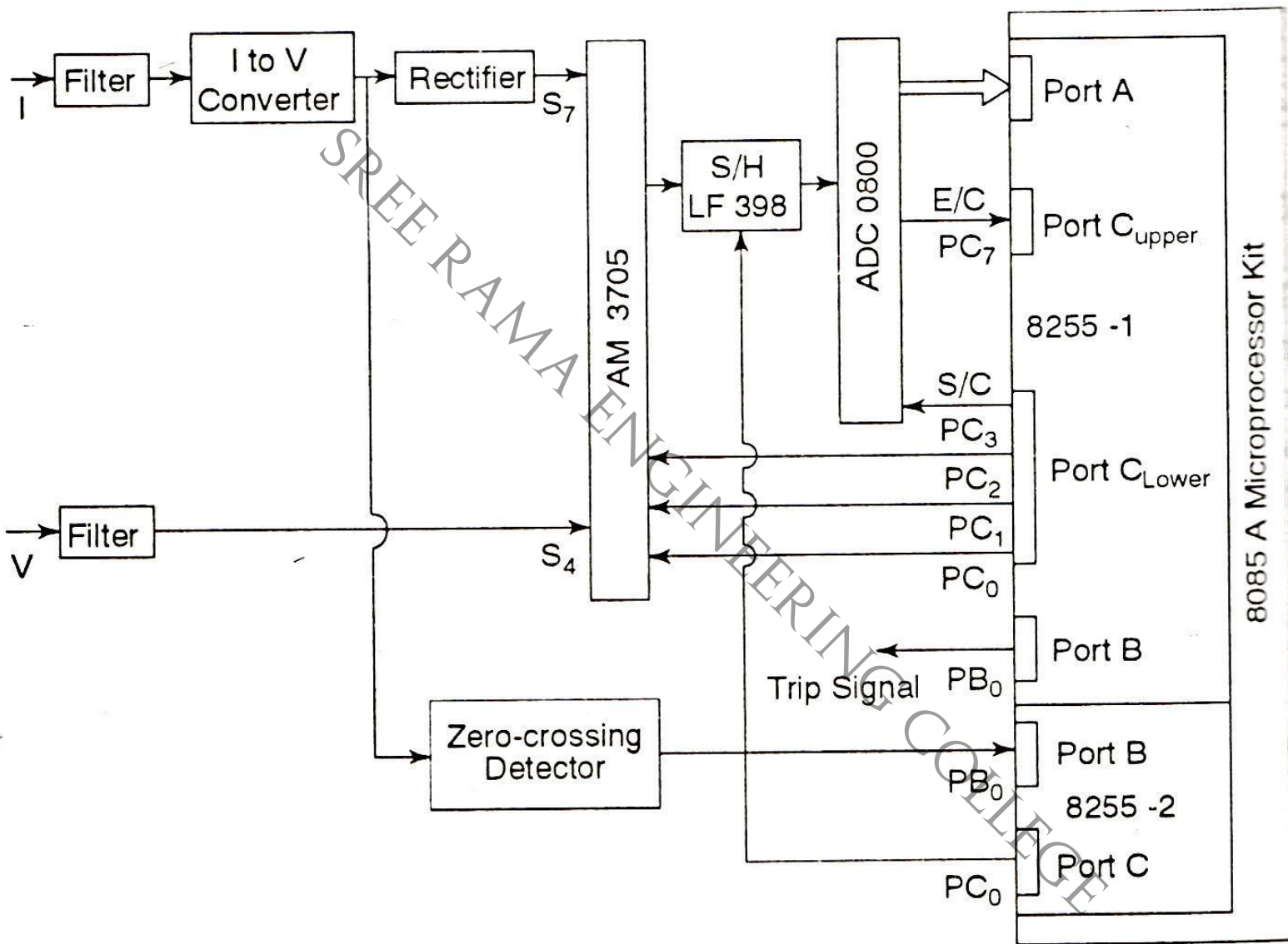
FIGURE 8.9 Block schematic diagram of interface for reactance relay
