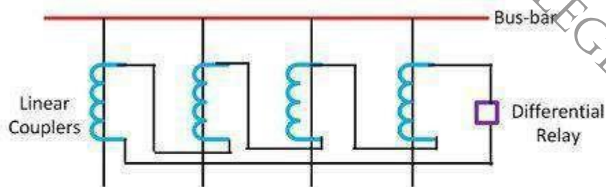
Voltage Differential Relaying For Bus-bar
